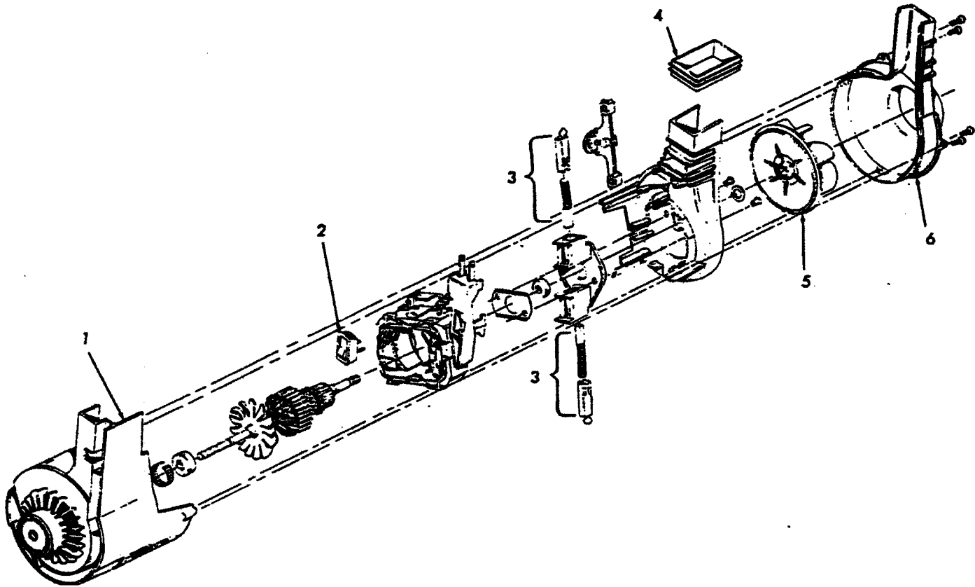
Motor Assembly - 43576102
